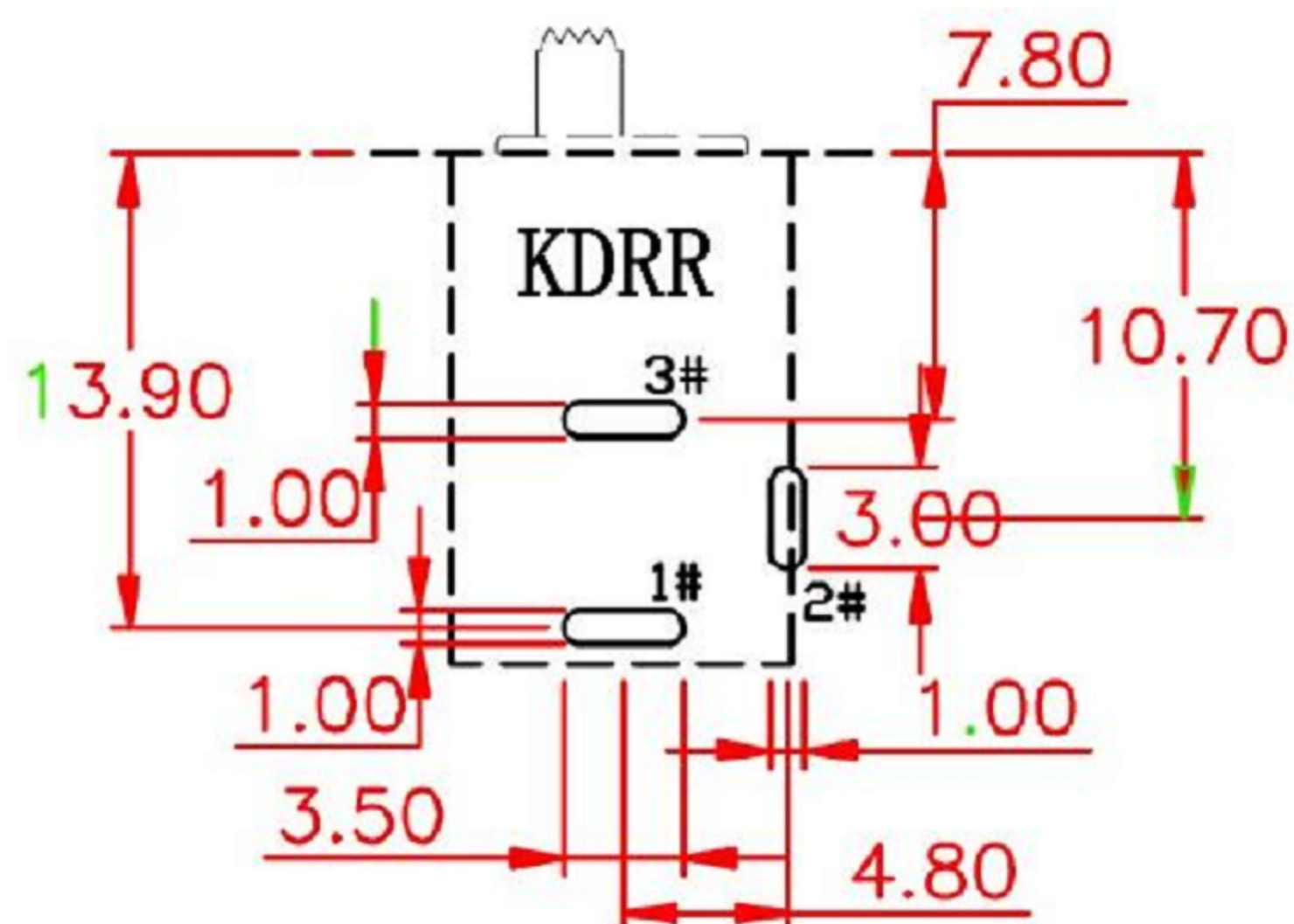
P. C. B LAYOUT BOTTOM VIEW
